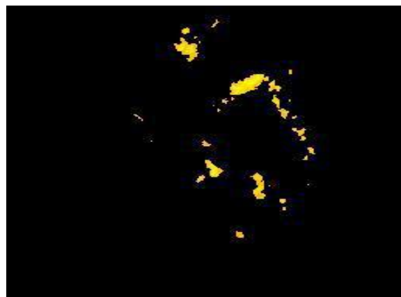
Fig 6: Segmented Image
